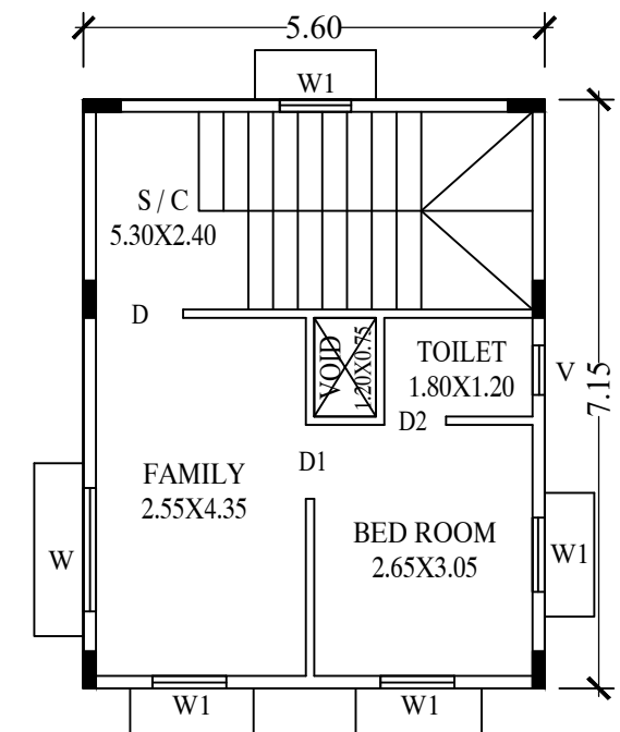
PROPOSED FIRST & SECOND FLOOR PLAN
